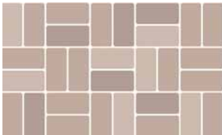
Block- und Parkettverband · block- and parquet bond
